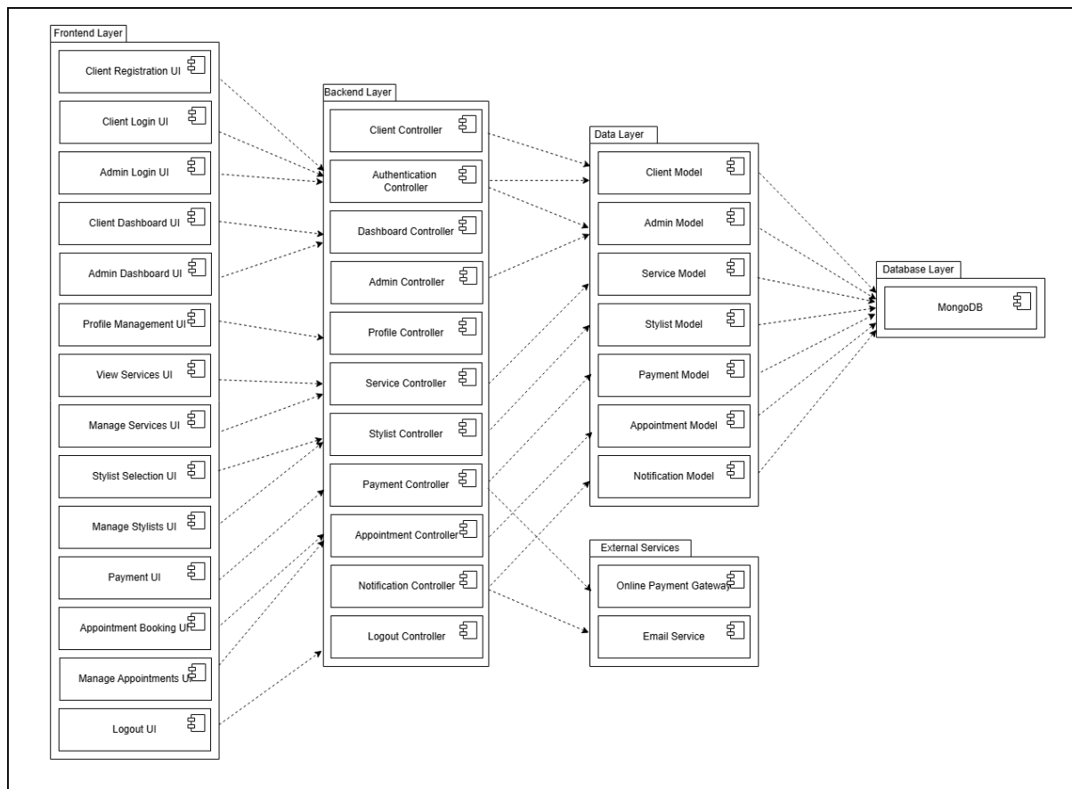
Figure 22: Component Diagram
